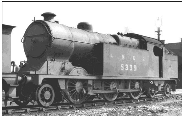
LNER class L1 2-6-4T no.5339
